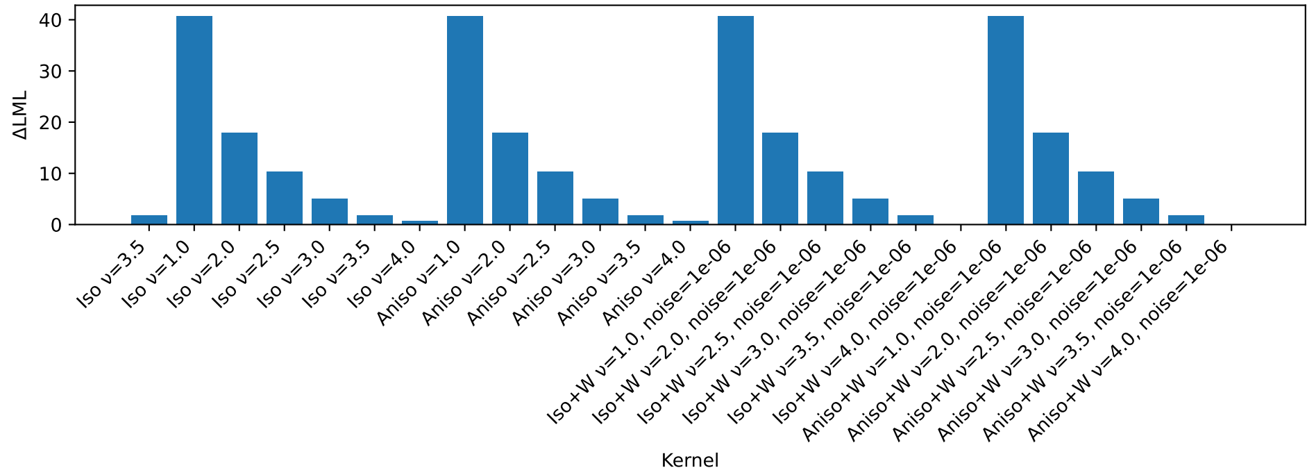
Difference from best LML (T2)
