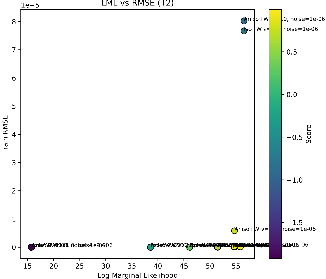
LML vs RMSE (T2)
